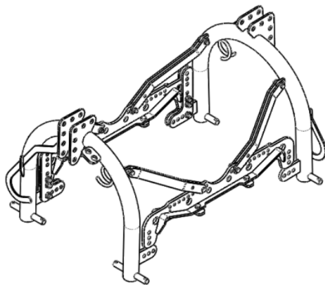
Dreipunkt Beidseitig Front/- Heckanbau Three-Point linkage for rear and front attachment Arceau à trois-point court
