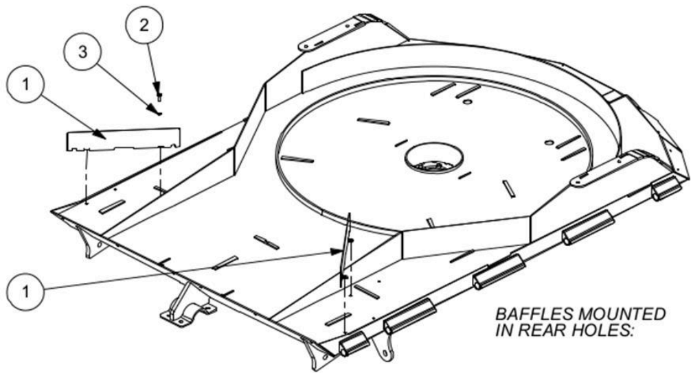
BAFFLE POSITIONS FITTED TO MC630 CENTRE DECK:
