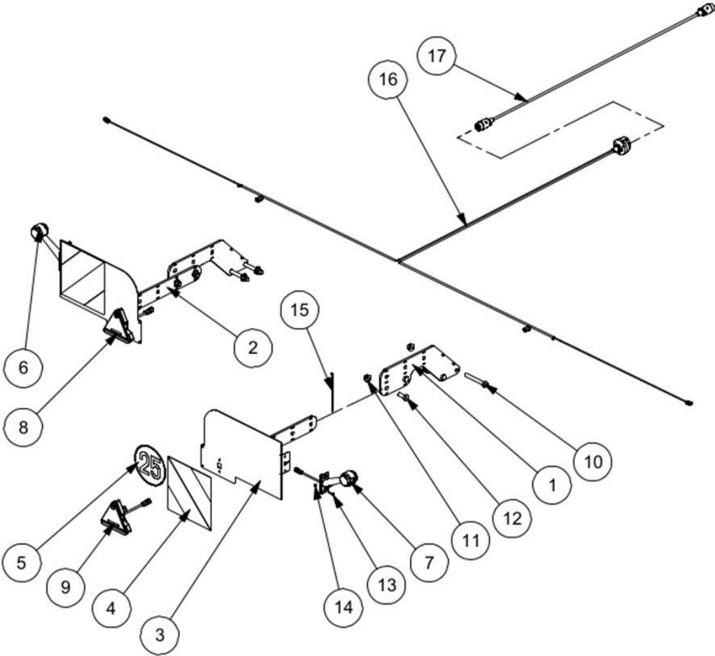
MARKER BOARD POSITION FOR MC470:
